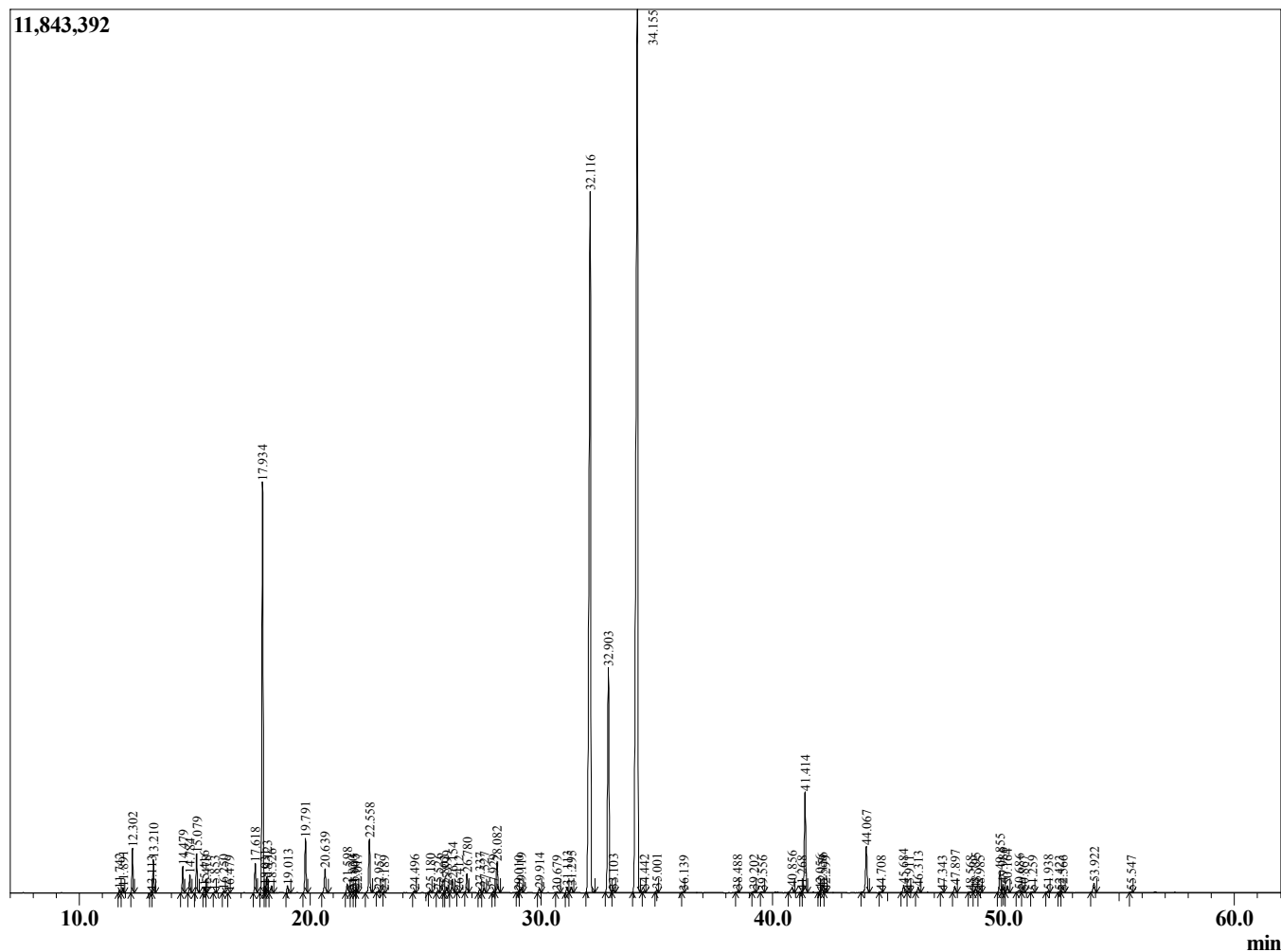
Chromatogram Cymbopogon citratus
